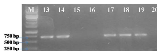
Fig. 3. Detection of ToLCV through PCR in infected calendula plants from different locations using TLCV1-F/R. M- Molecular marker (1 Kb ladder), Lane – 13, 14, 17, 18 & 19: 770 bp DNA specific to coat protein region, Lane – 15, 16 & 20- no amplification
