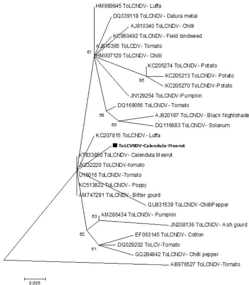
Fig. 4. Phylogenetic tree depicting the relationship of various begomoviruses based on alignment of coat protein gene nucleotide sequences. Tree was constructed using Mega 5 programme with 1000 bootstrap values
