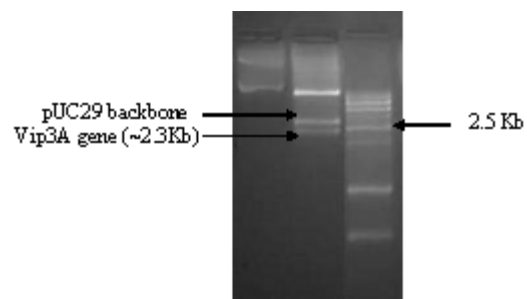
Fig. 3. Restriction digestion (NdeI/XhoI) of pUC29-Vip3a Clone
