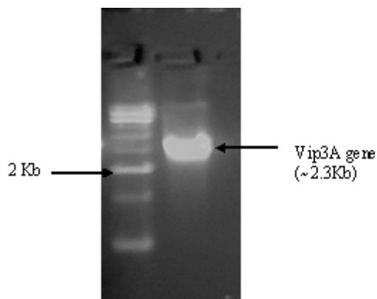
Fig. 2. PCR Amplified Vip3A gene from NBAIR-BTEG1 loaded on 1% Agarose Gel
