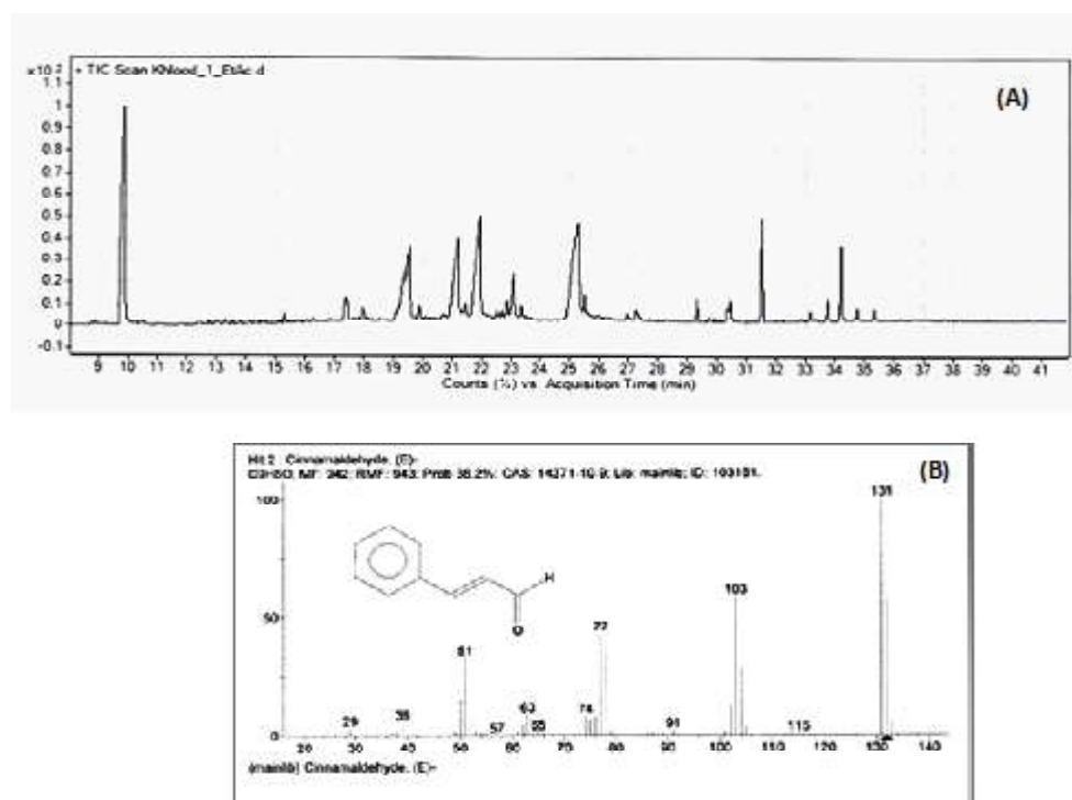
Fig. 9. Gas Chromatography-Mass Spectra showing the major peak in GC analysis (A) and identified compound “cinnamaldehyde” in Mass Spectral analysis (B)
