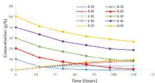
Fig. 3. The effects on glycerol consumption and ethanol production of the initial glycerol concentration during the fermentation of E. aerogenes at 37 °C for 120 hours
